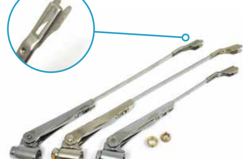
Pre-war pattern, for 3/16" or 1/4" shaft slot & peg blade fitting 477PRE-N, 477PRE-AC, 477PRE-BC
