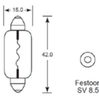
Festoon 15 x 44mm
