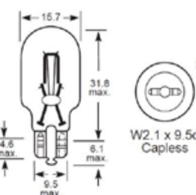
T15 Capless Wedge
