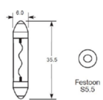
Festoon 6 x 36mm & 8 x 36mm
