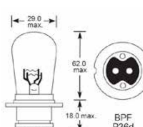
British Pre Focus SC P36D
