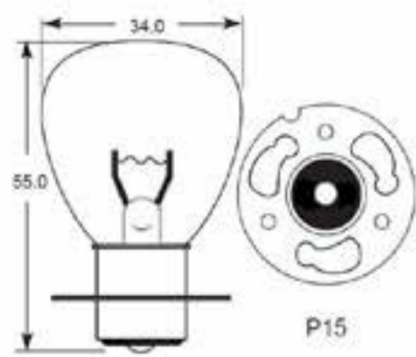
American Pre-Focus APF P13S 30
