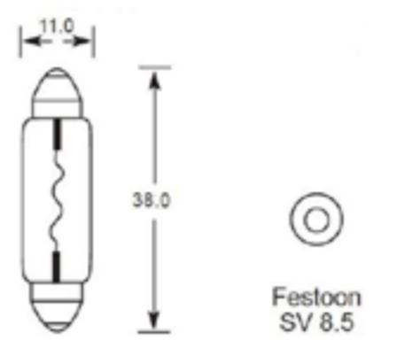
Festoon 11 x 39mm
